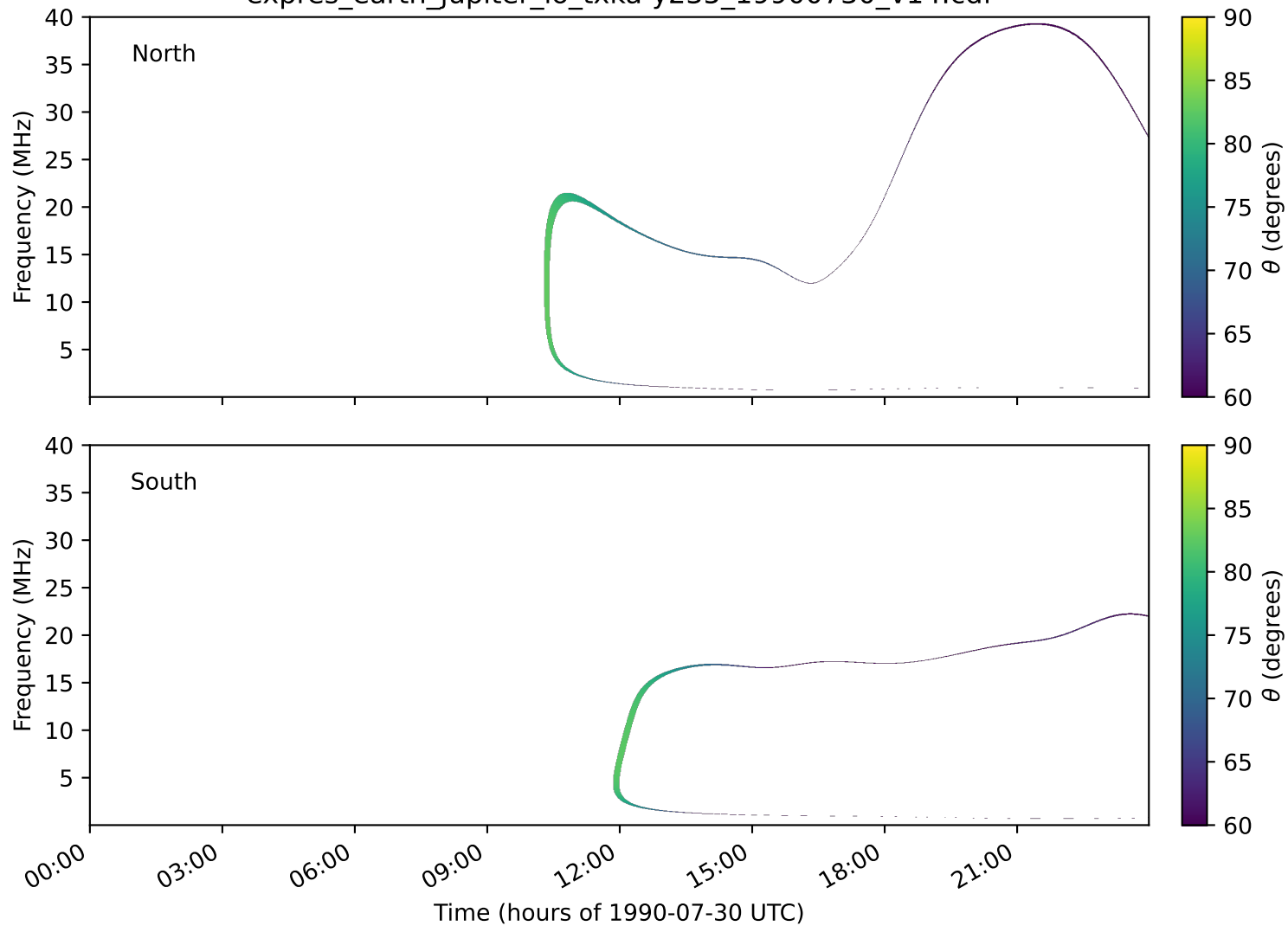
expres_earth_jupiter_io_txka-y235_19900730_v14.cdf
