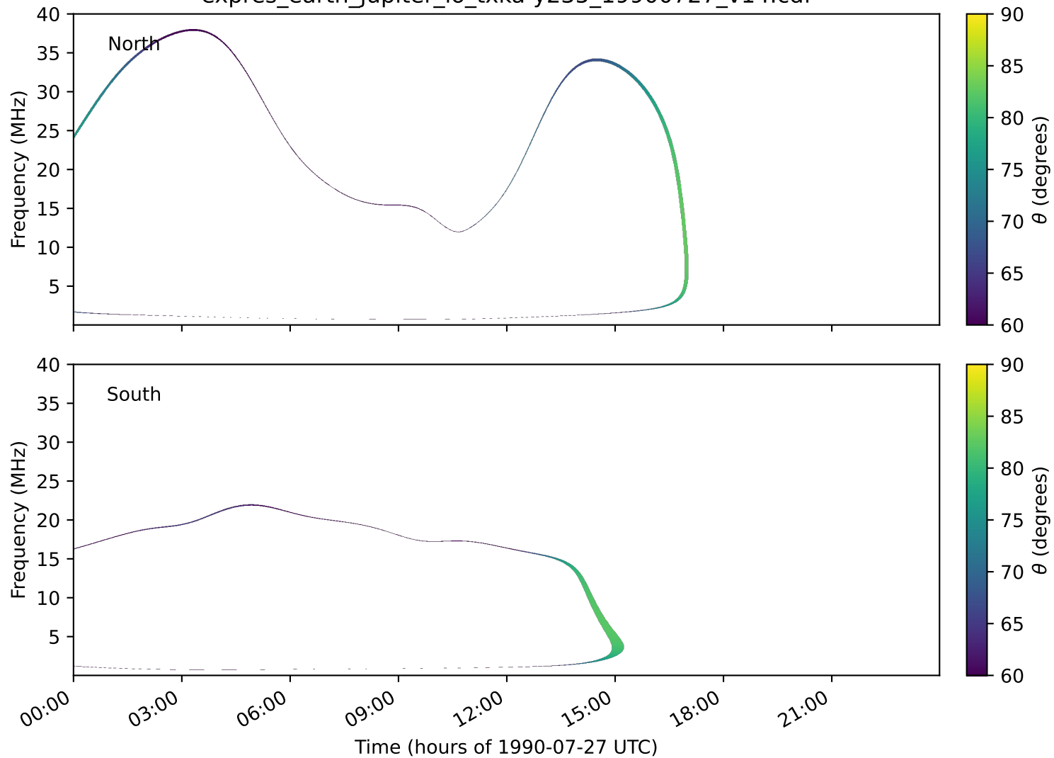
expres_earth_jupiter_io_txka-y235_19900727_v14.cdf
