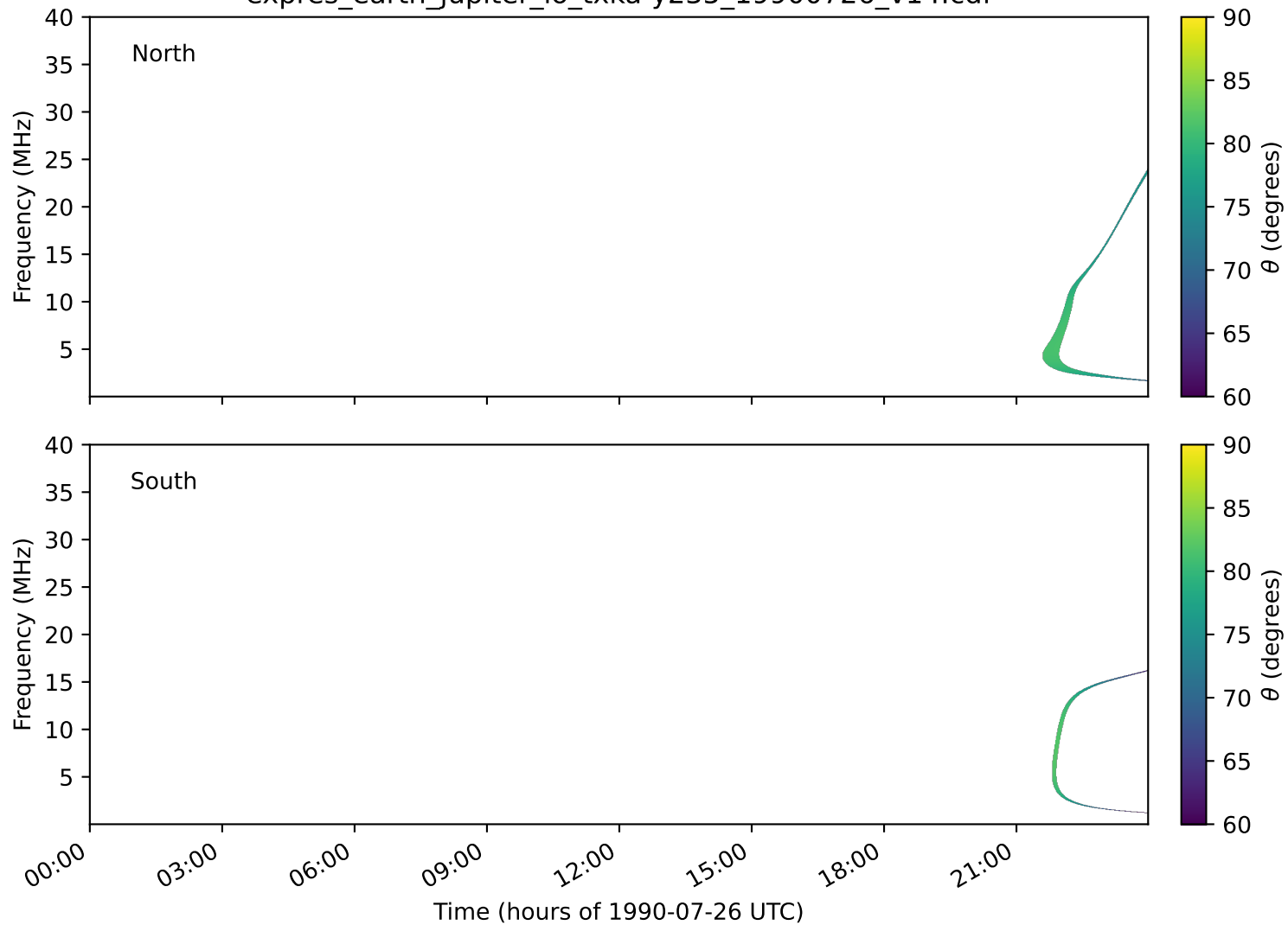
expres_earth_jupiter_io_txka-y235_19900726_v14.cdf
