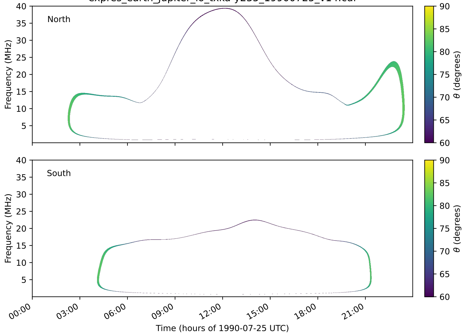
expres_earth_jupiter_io_txka-y235_19900725_v14.cdf
