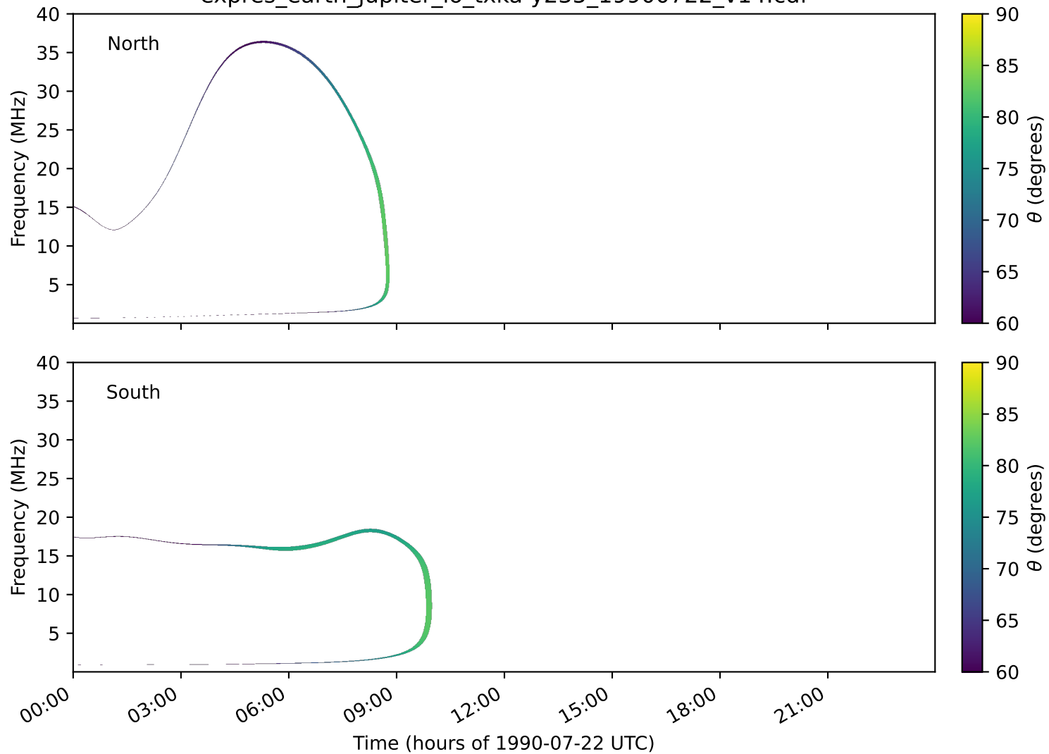
expres_earth_jupiter_io_txka-y235_19900722_v14.cdf
