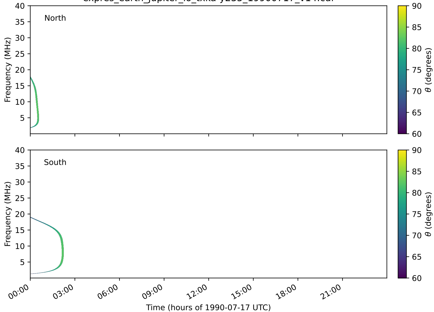
expres_earth_jupiter_io_txka-y235_19900717_v14.cdf
