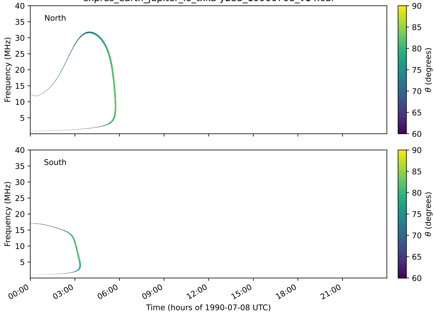
expres_earth_jupiter_io_txka-y235_19900708_v14.cdf
