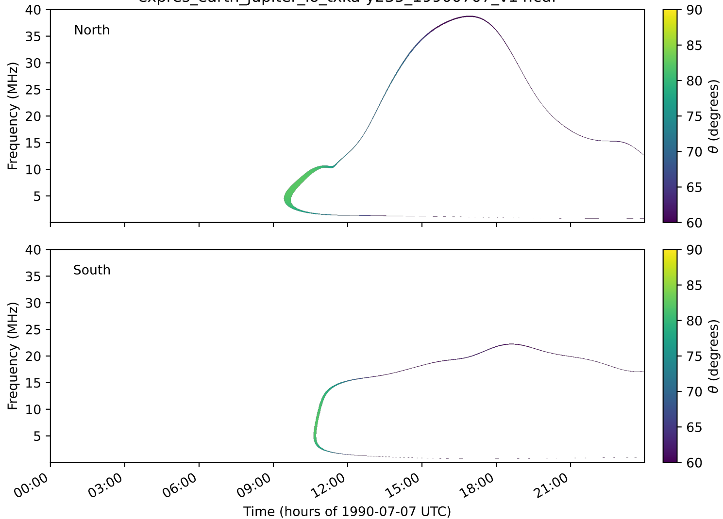
expres_earth_jupiter_io_txka-y235_19900707_v14.cdf
