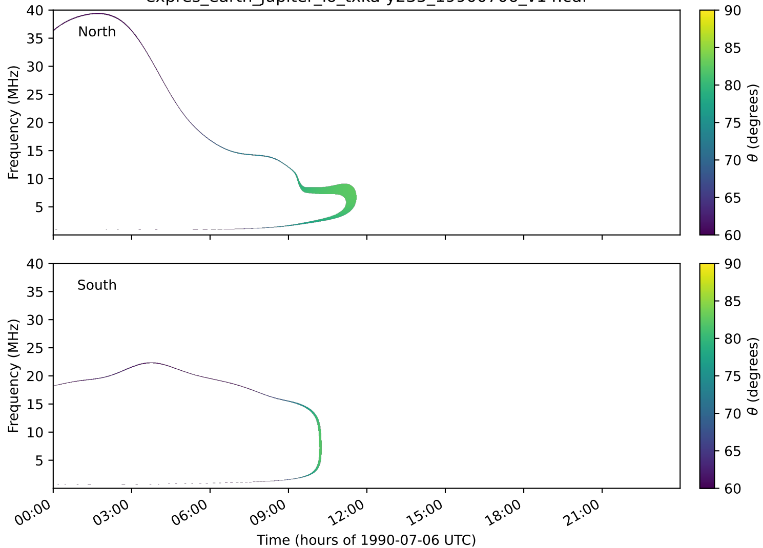
expres_earth_jupiter_io_txka-y235_19900706_v14.cdf
