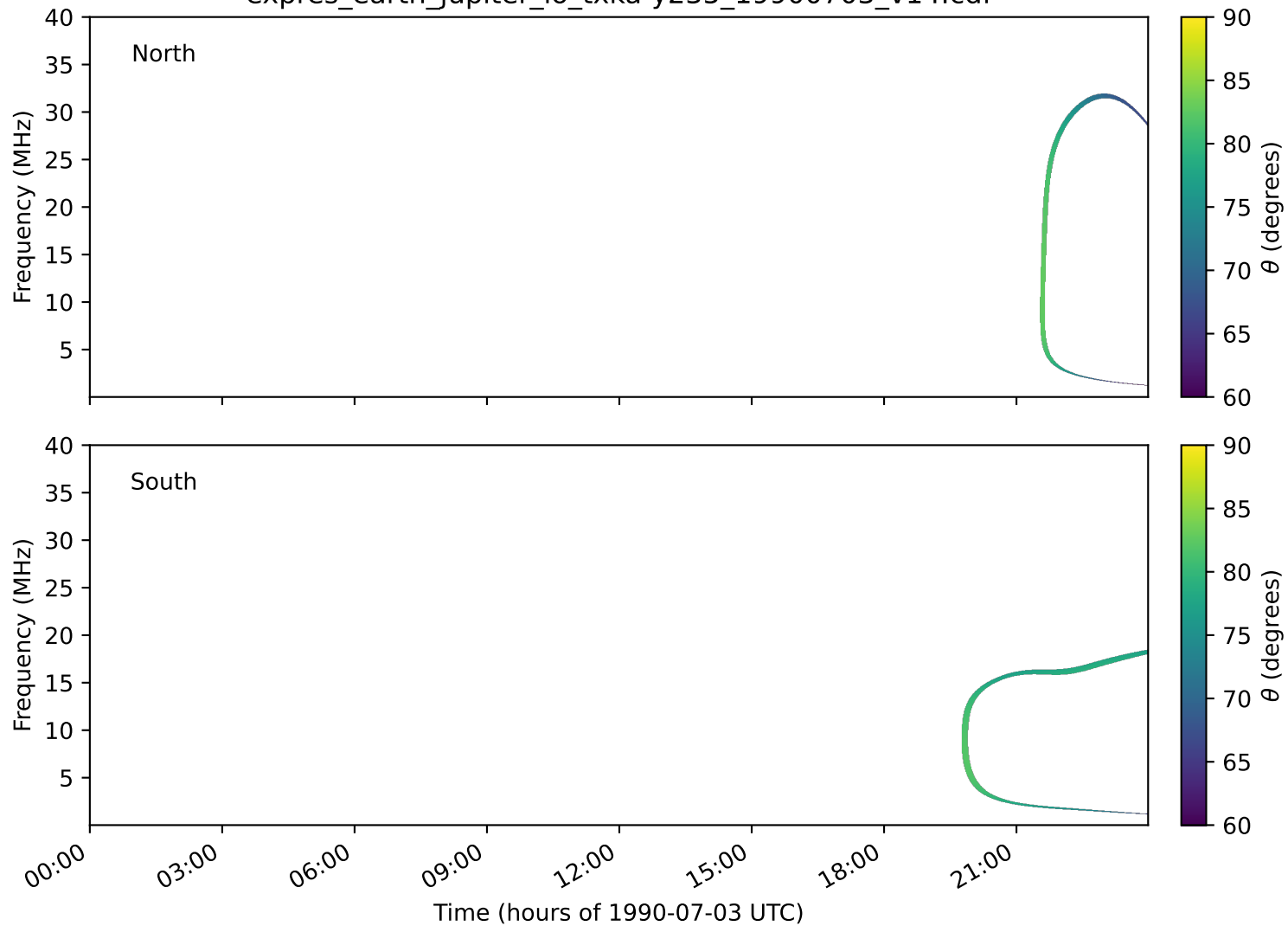
expres_earth_jupiter_io_txka-y235_19900703_v14.cdf
