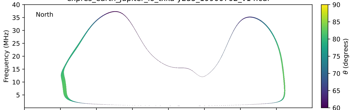
expres_earth_jupiter_io_txka-y235_19900702_v14.cdf
