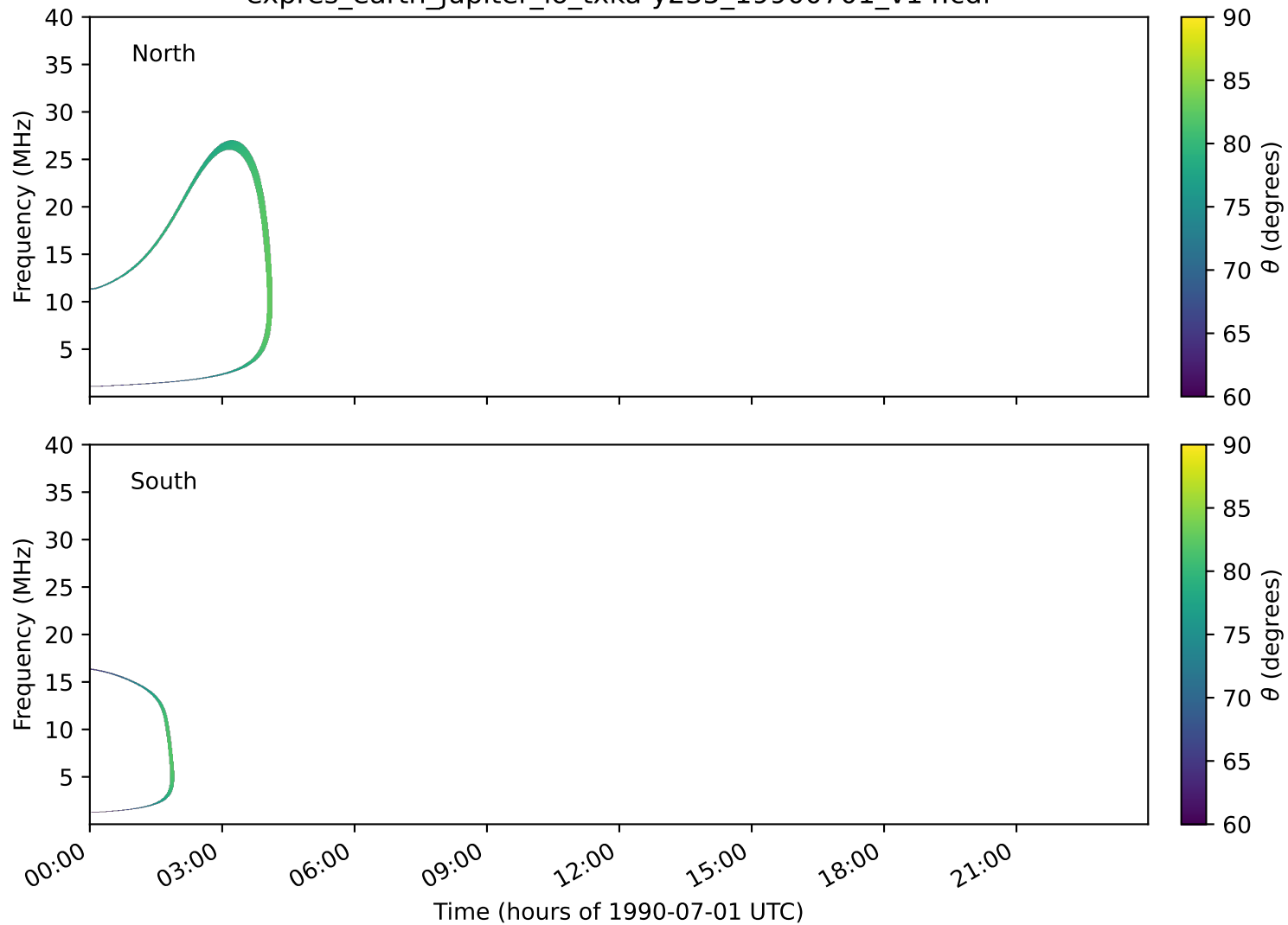
expres_earth_jupiter_io_txka-y235_19900701_v14.cdf
