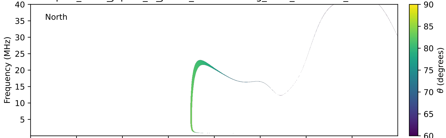
expres_earth_jupiter_io_jrm33_lossc-wid1deg_3kev_19900730_v11.cdf
