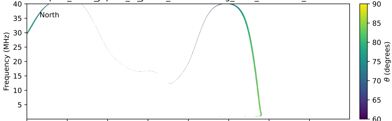
expres_earth_jupiter_io_jrm33_lossc-wid1deg_3kev_19900727_v11.cdf
