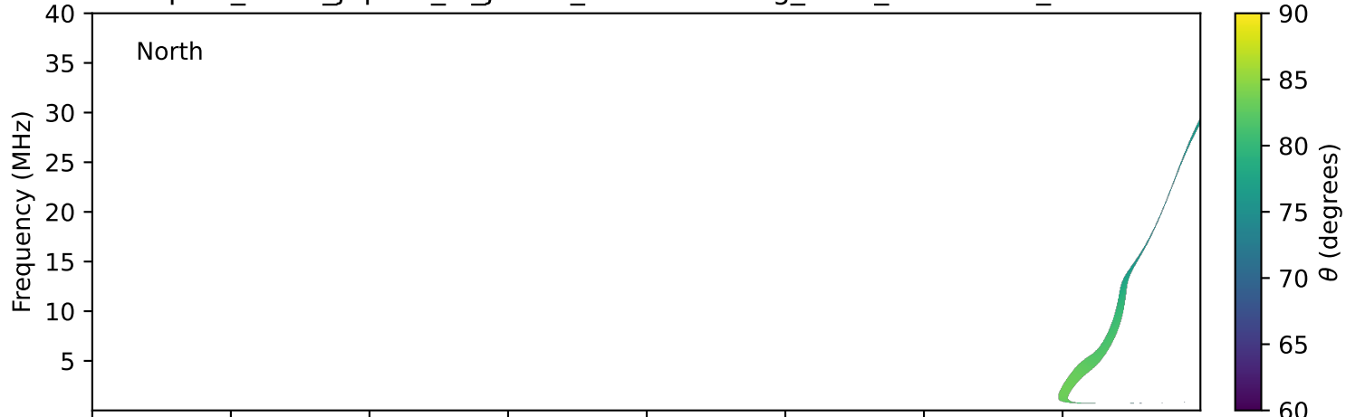
expres_earth_jupiter_io_jrm33_lossc-wid1deg_3kev_19900726_v11.cdf
