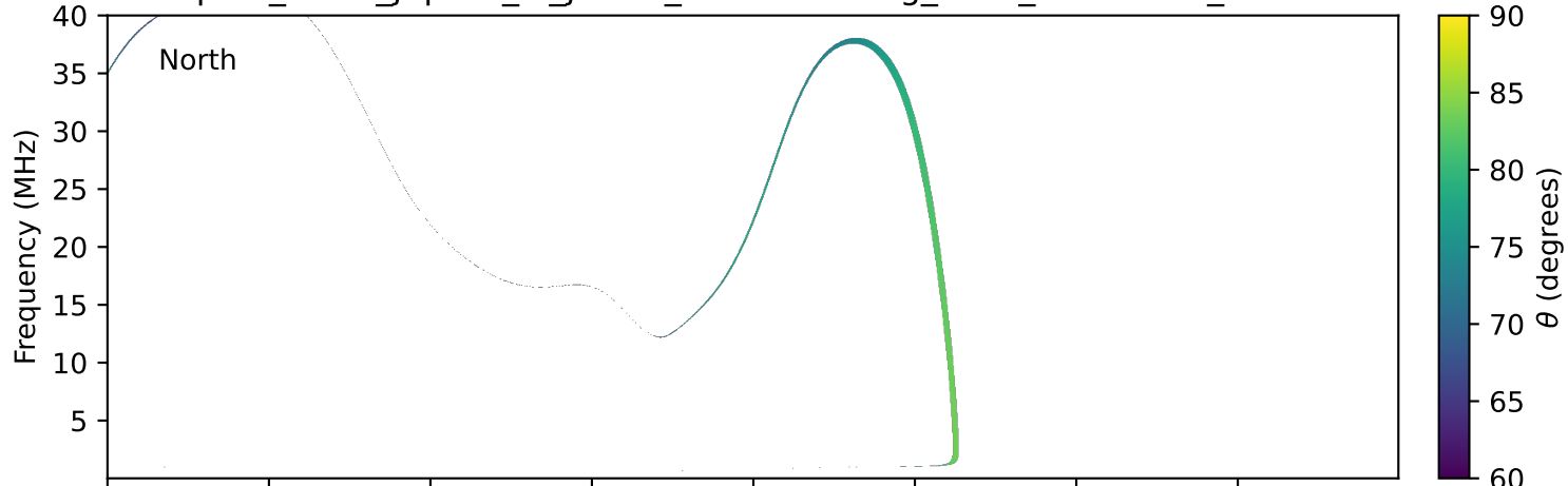
expres_earth_jupiter_io_jrm33_lossc-wid1deg_3kev_19900720_v11.cdf
