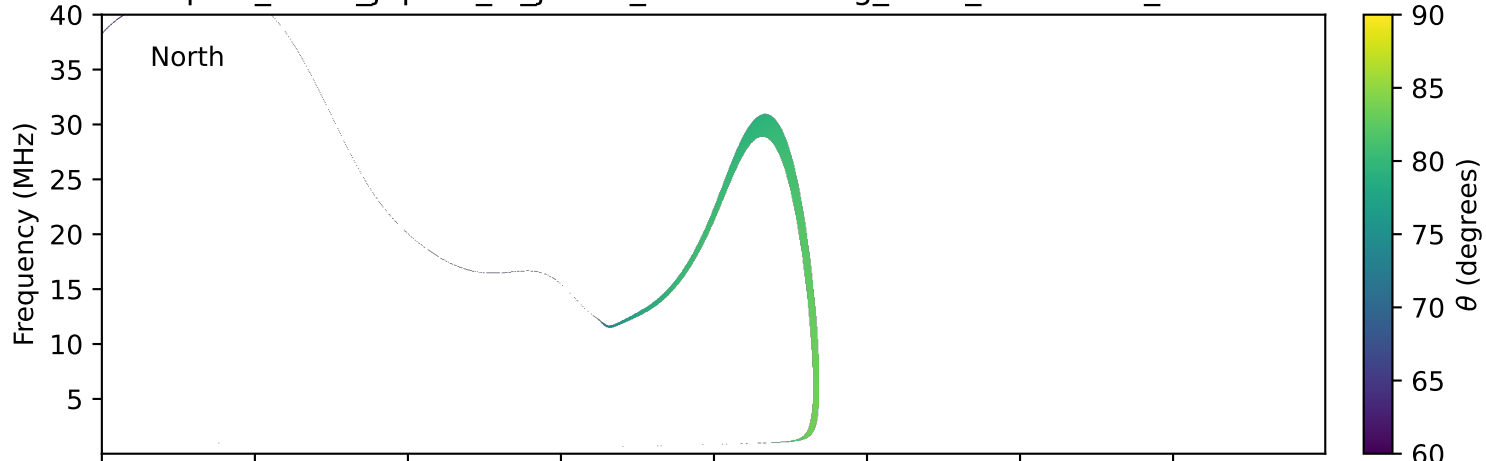
expres_earth_jupiter_io_jrm33_lossc-wid1deg_3kev_19900713_v11.cdf
