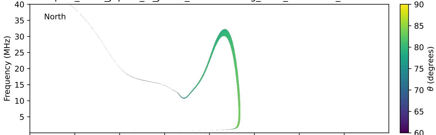
expres_earth_jupiter_io_jrm09_lossc-wid1deg_3kev_19900713_v11.cdf
