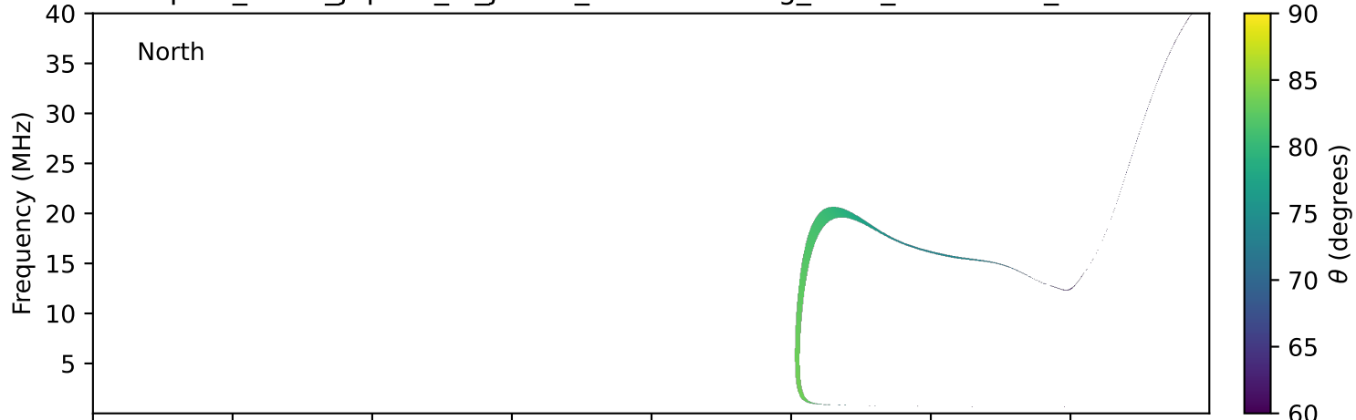
expres_earth_jupiter_io_jrm09_lossc-wid1deg_3kev_19900705_v11.cdf
