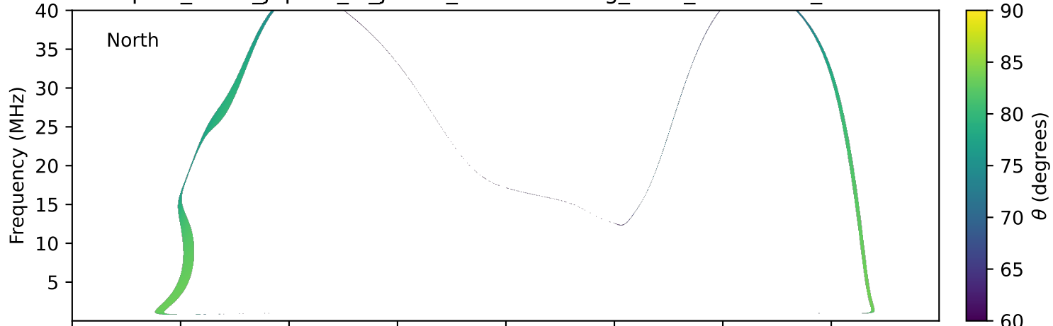
expres_earth_jupiter_io_jrm09_lossc-wid1deg_3kev_19900702_v11.cdf
