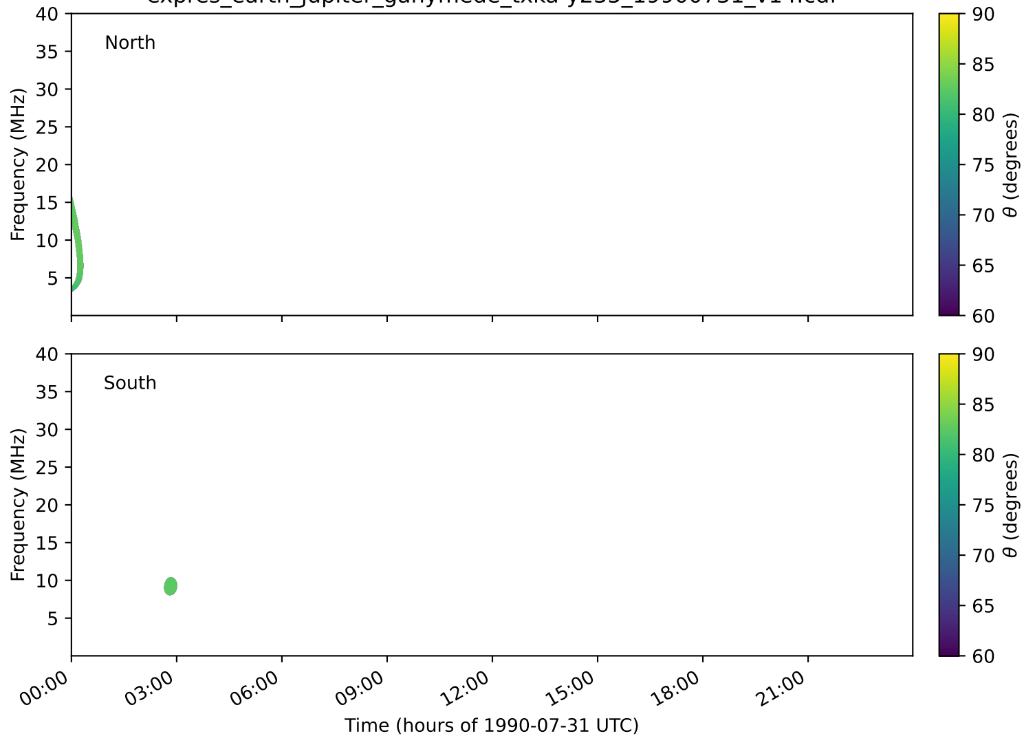
expres_earth_jupiter_ganymede_txka-y235_19900731_v14.cdf
