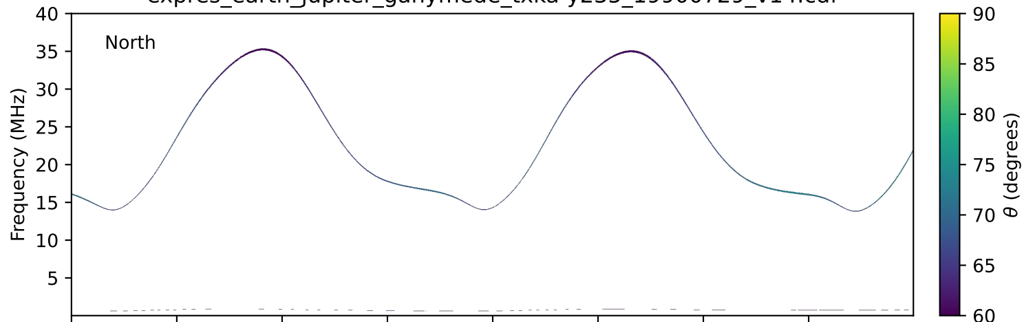
expres_earth_jupiter_ganymede_txka-y235_19900729_v14.cdf
