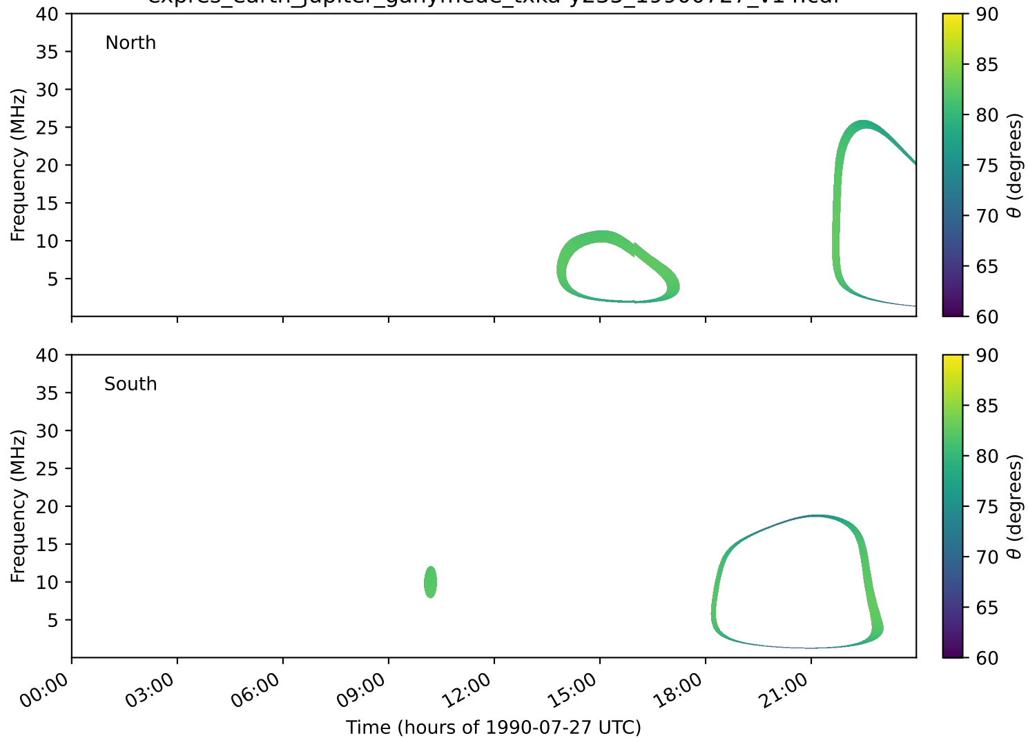
expres_earth_jupiter_ganymede_txka-y235_19900727_v14.cdf
