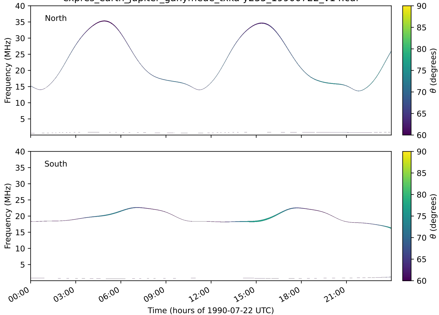
expres_earth_jupiter_ganymede_txka-y235_19900722_v14.cdf
