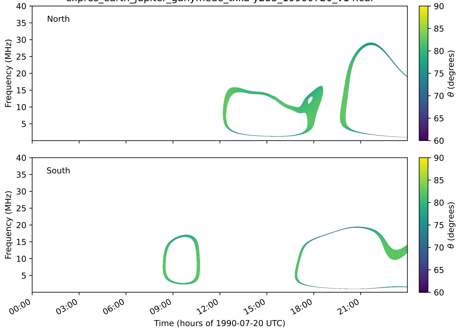
expres_earth_jupiter_ganymede_txka-y235_19900720_v14.cdf
