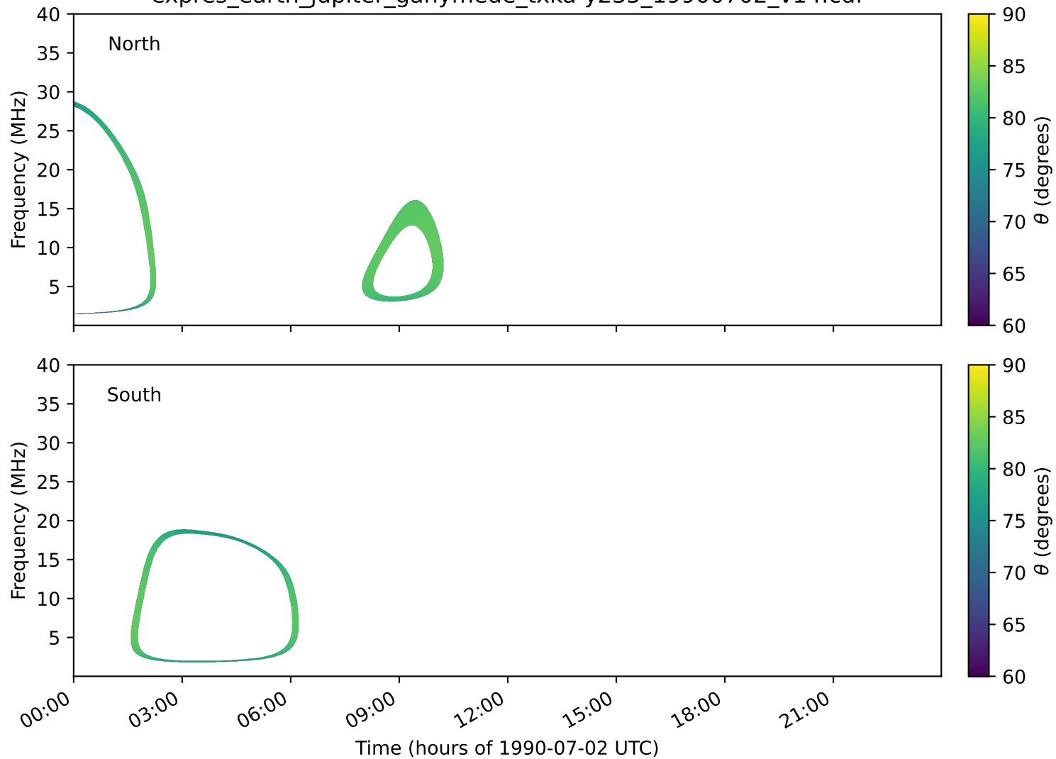
expres_earth_jupiter_ganymede_txka-y235_19900702_v14.cdf
