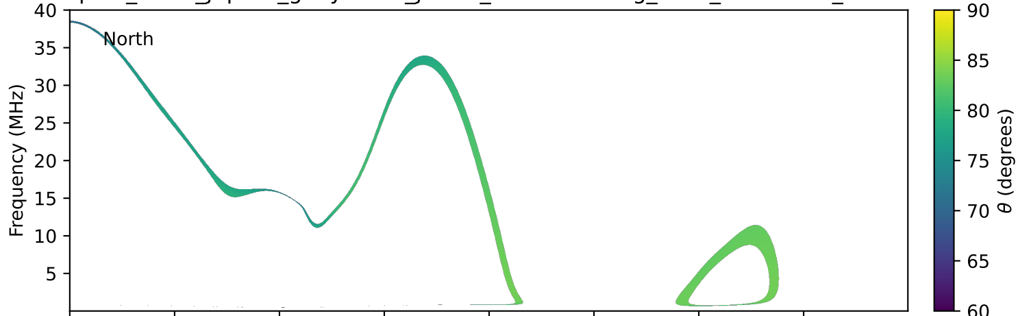
expres_earth_jupiter_ganymede_jrm09_lossc-wid1deg_3kev_19900709_v11.cdf
