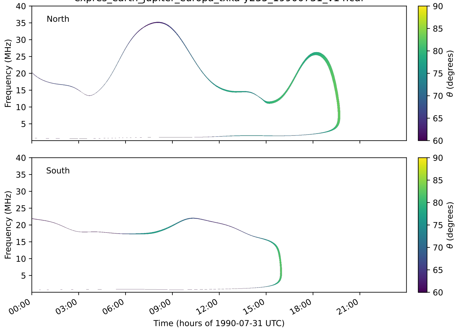
expres_earth_jupiter_europa_txka-y235_19900731_v14.cdf
