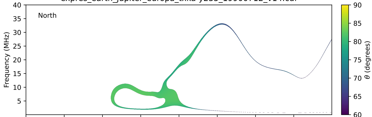
expres_earth_jupiter_europa_txka-y235_19900712_v14.cdf
