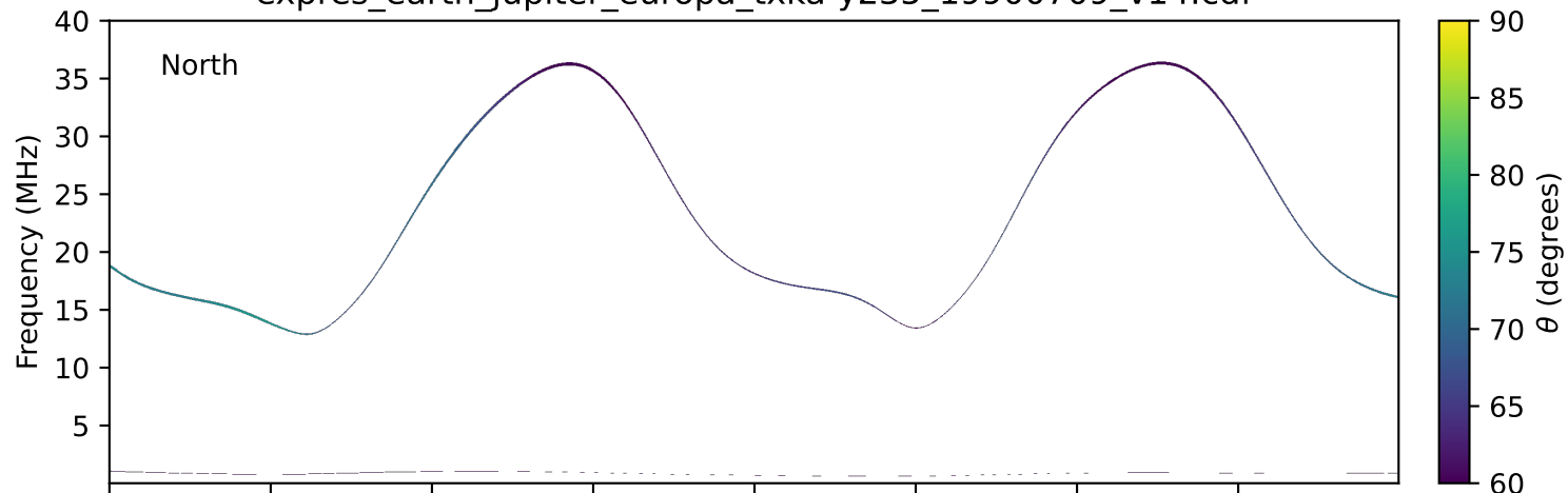
expres_earth_jupiter_europa_txka-y235_19900709_v14.cdf
