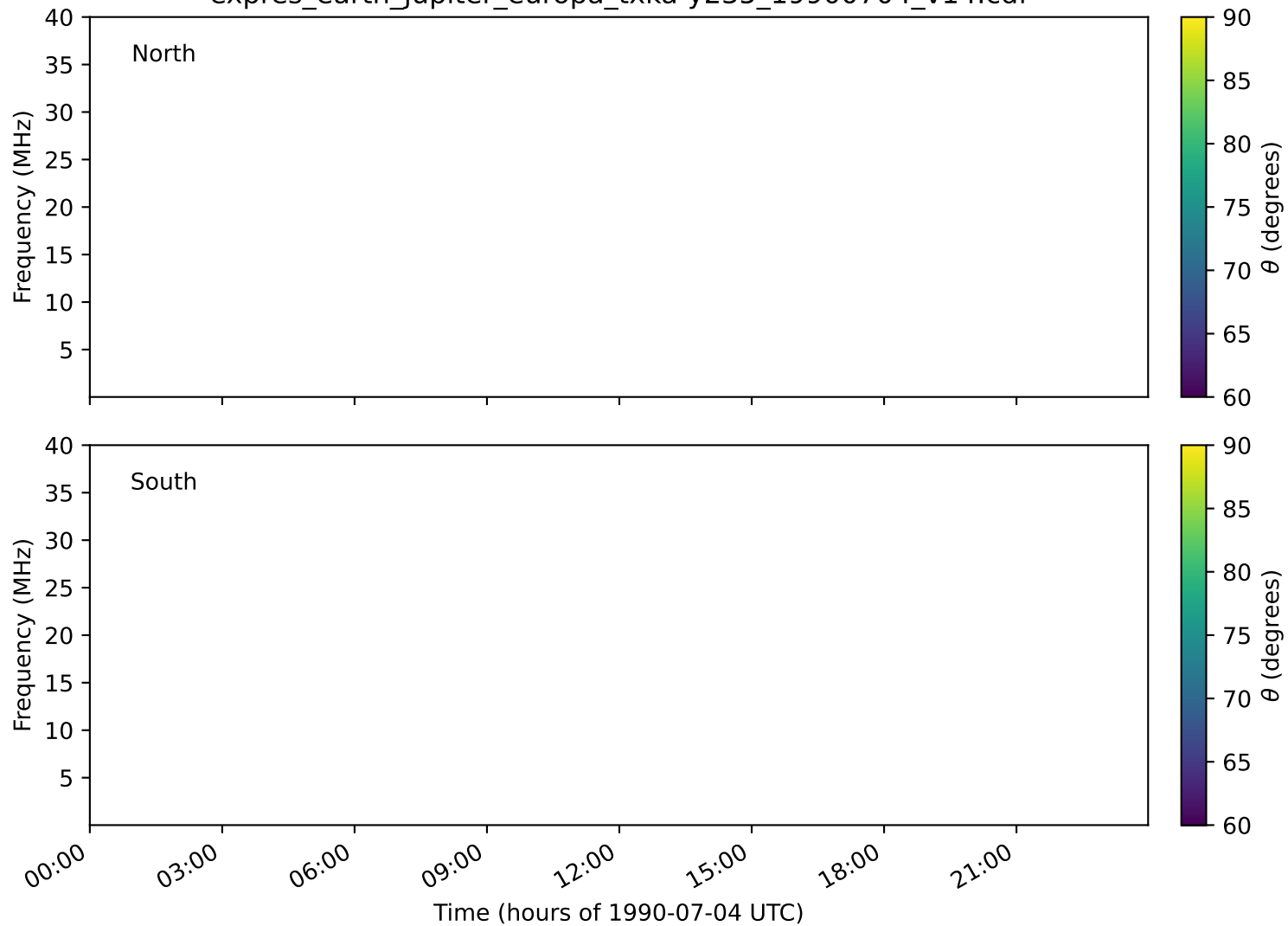
expres_earth_jupiter_europa_txka-y235_19900704_v14.cdf
