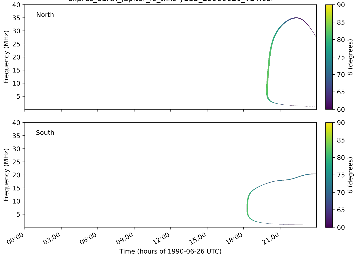
expres_earth_jupiter_io_txka-y235_19900626_v14.cdf
