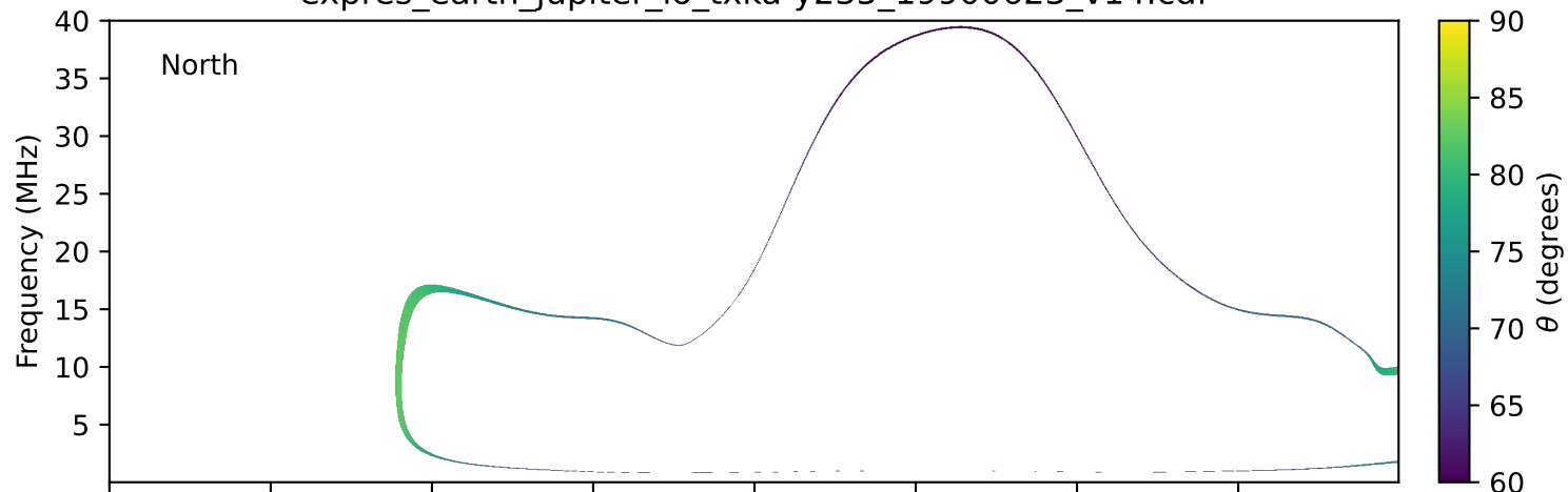
expres_earth_jupiter_io_txka-y235_19900623_v14.cdf
