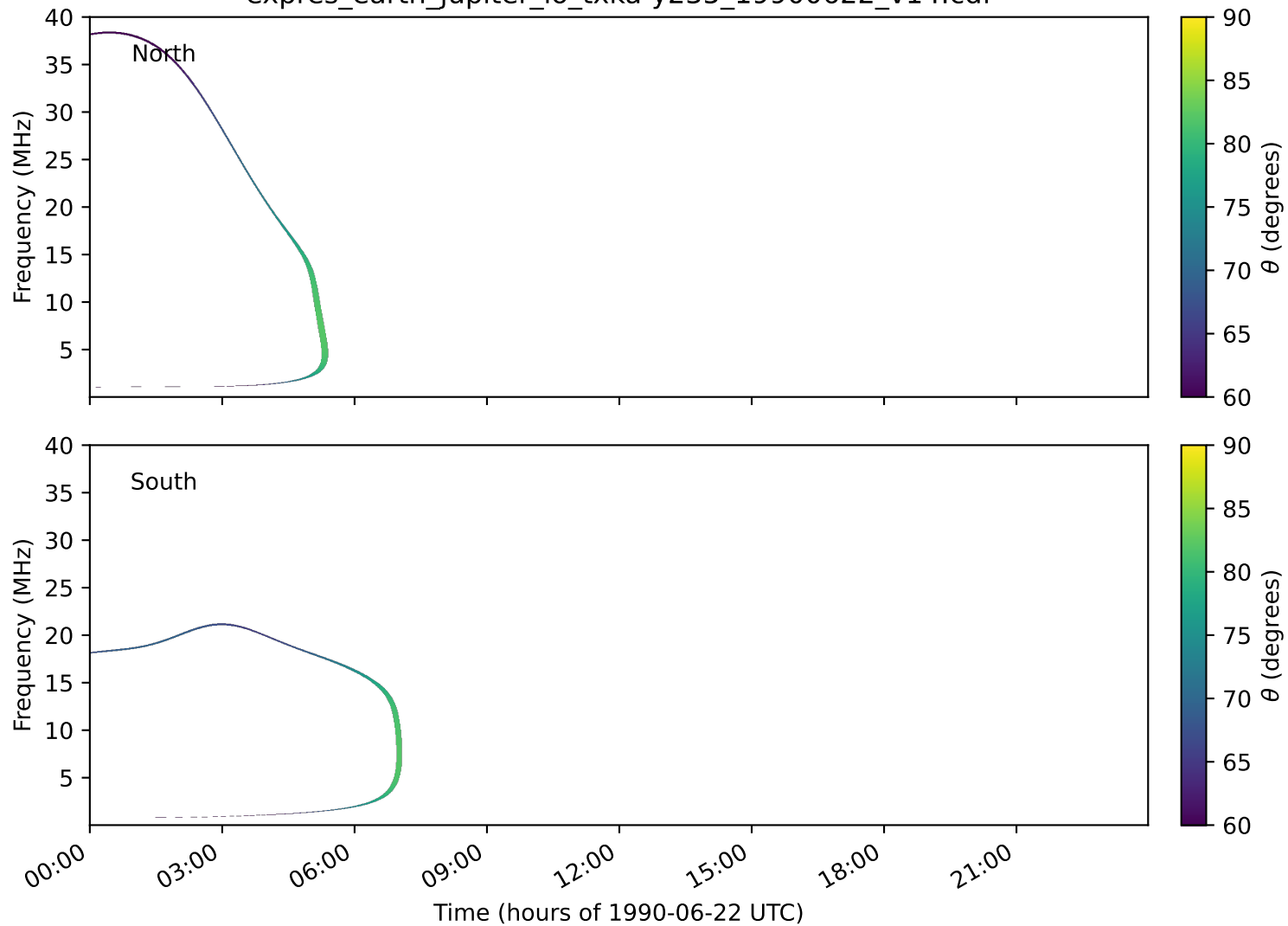
expres_earth_jupiter_io_txka-y235_19900622_v14.cdf
