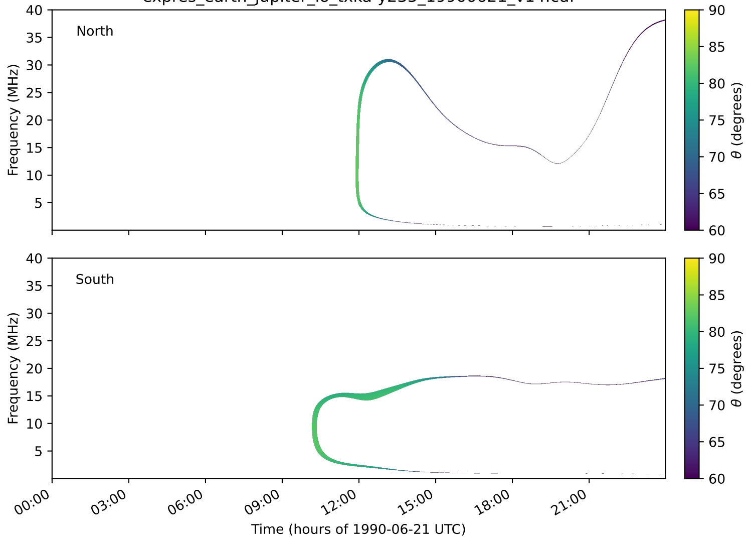
expres_earth_jupiter_io_txka-y235_19900621_v14.cdf
