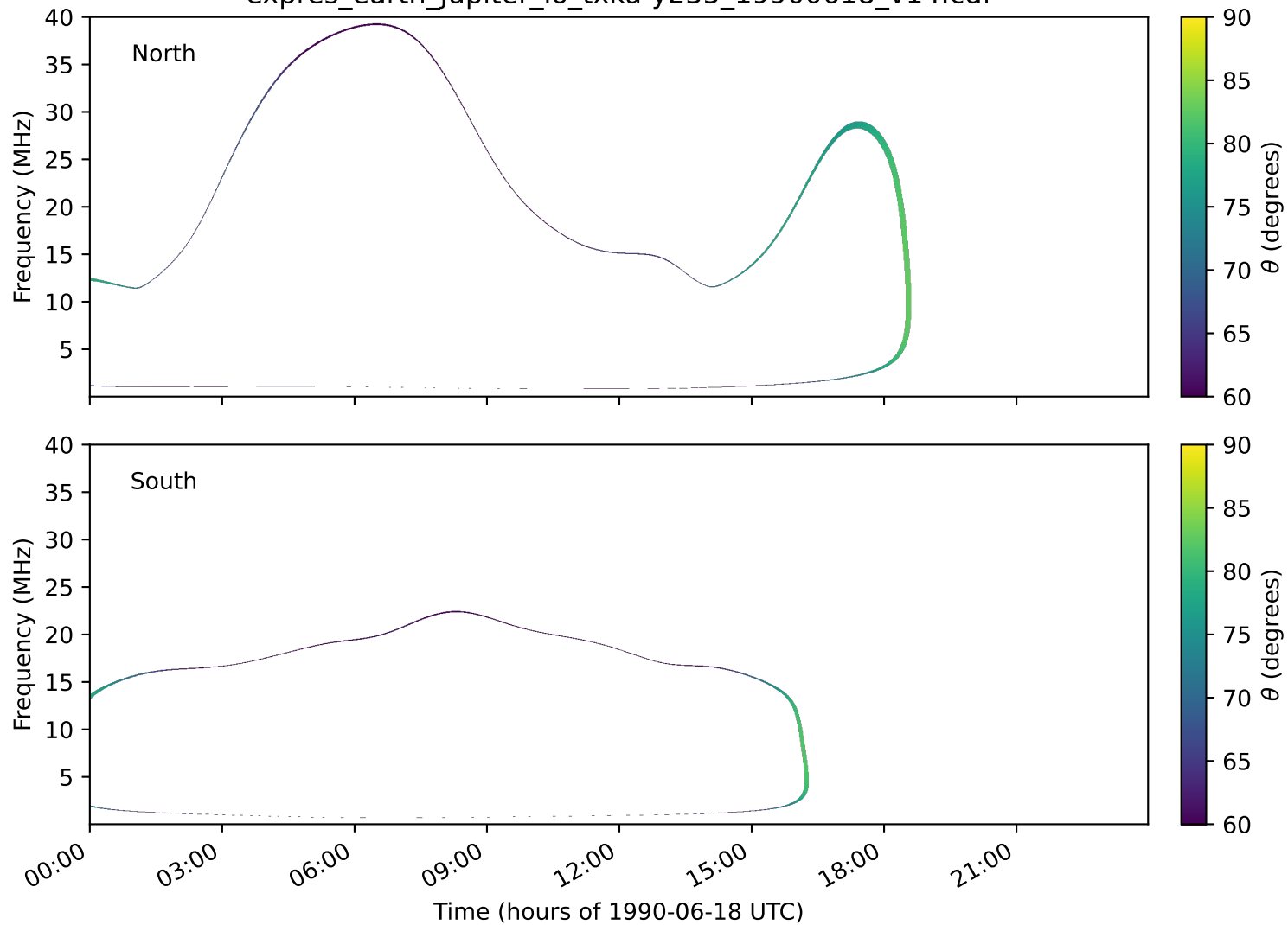
expres_earth_jupiter_io_txka-y235_19900618_v14.cdf
