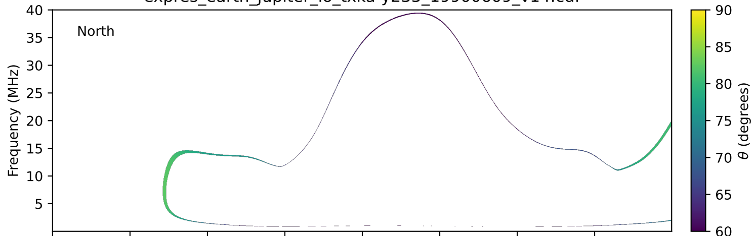
expres_earth_jupiter_io_txka-y235_19900609_v14.cdf
