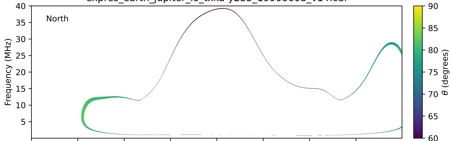
expres_earth_jupiter_io_txka-y235_19900608_v14.cdf
