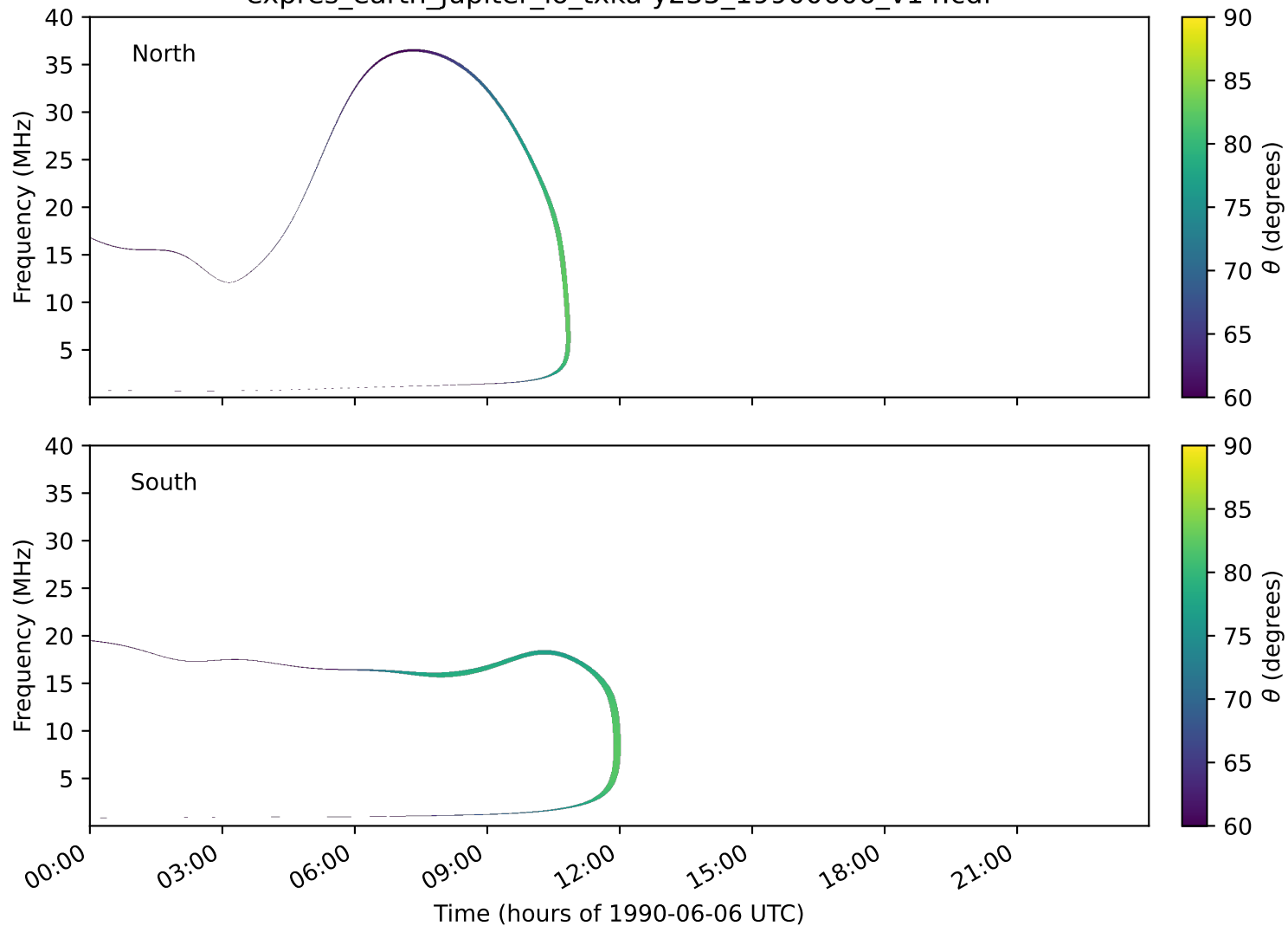
expres_earth_jupiter_io_txka-y235_19900606_v14.cdf
