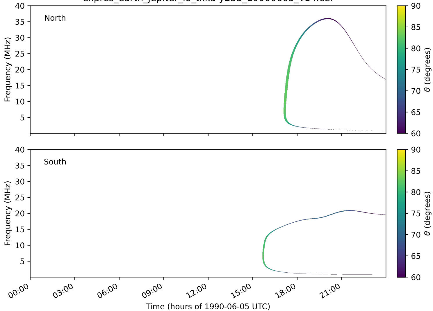
expres_earth_jupiter_io_txka-y235_19900605_v14.cdf
