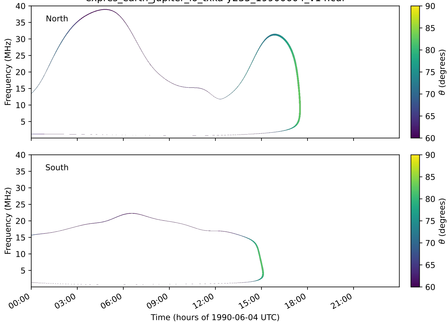
expres_earth_jupiter_io_txka-y235_19900604_v14.cdf
