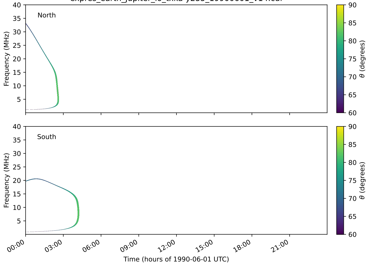
expres_earth_jupiter_io_txka-y235_19900601_v14.cdf
