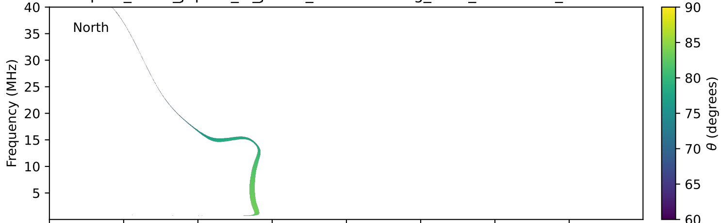
expres_earth_jupiter_io_jrm33_lossc-wid1deg_3kev_19900629_v11.cdf
