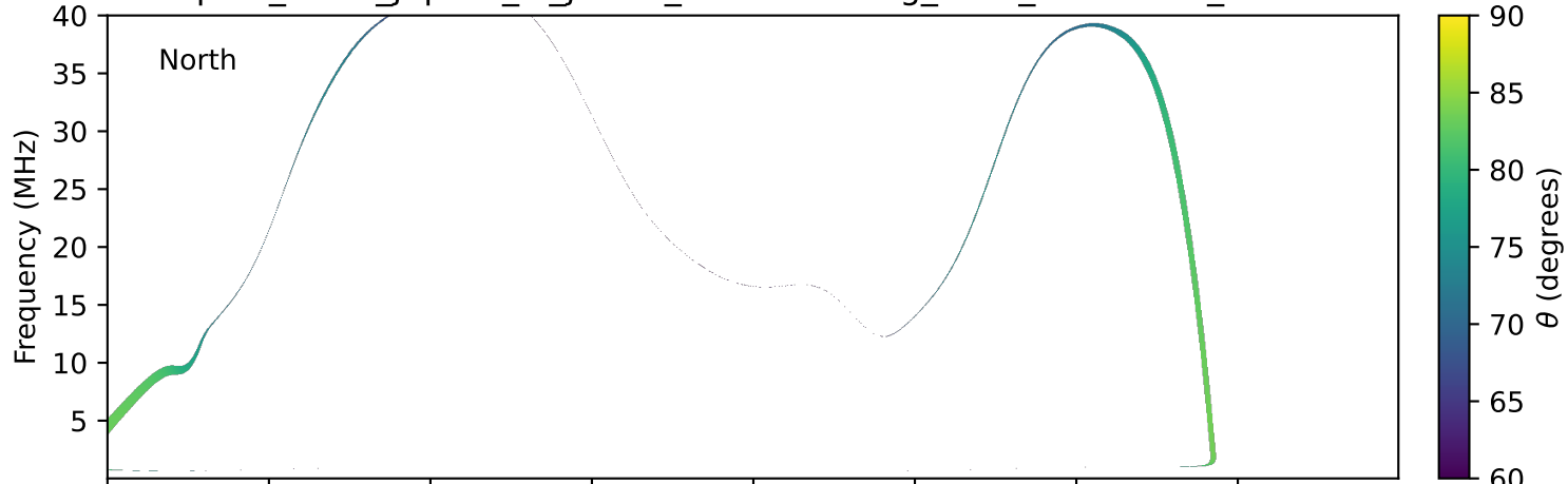
expres_earth_jupiter_io_jrm33_lossc-wid1deg_3kev_19900625_v11.cdf
