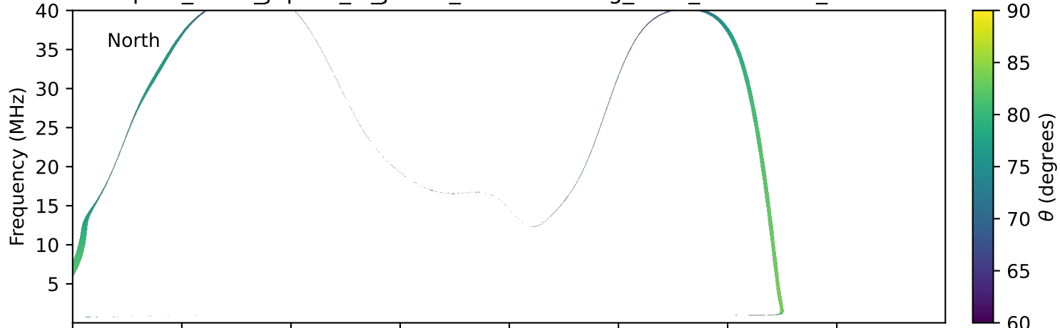
expres_earth_jupiter_io_jrm33_lossc-wid1deg_3kev_19900611_v11.cdf
