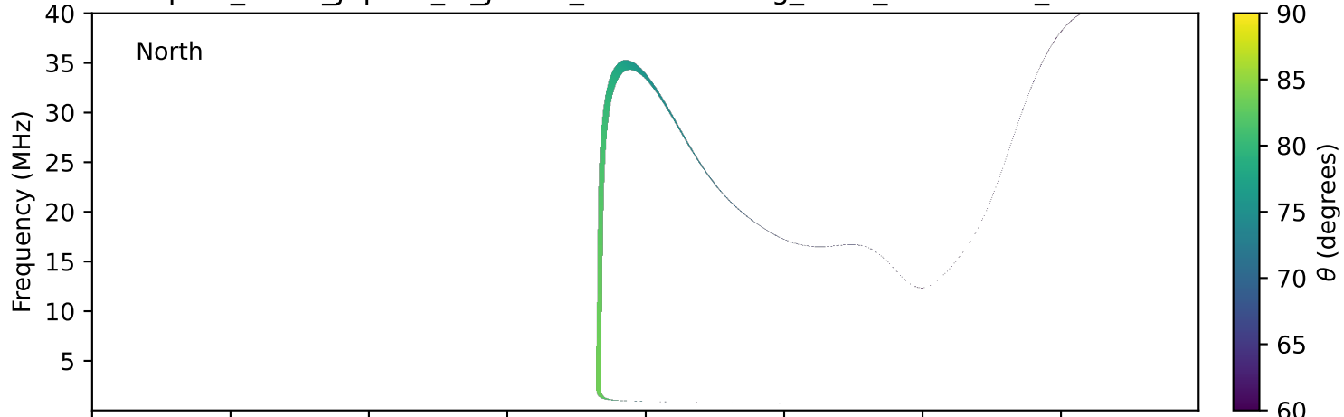
expres_earth_jupiter_io_jrm33_lossc-wid1deg_3kev_19900607_v11.cdf
