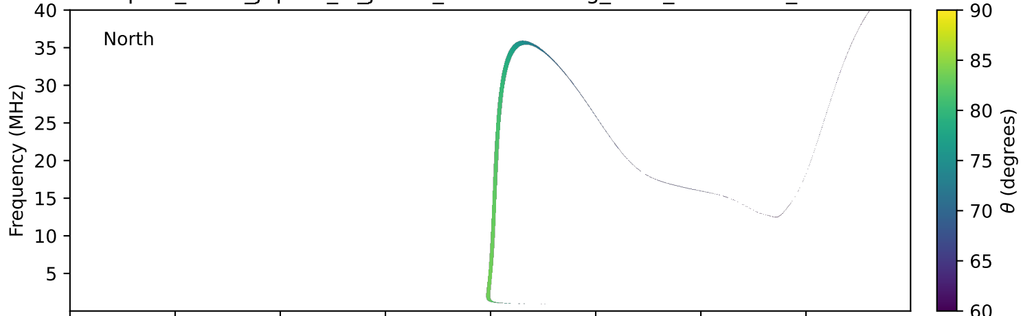
expres_earth_jupiter_io_jrm09_lossc-wid1deg_3kev_19900621_v11.cdf
