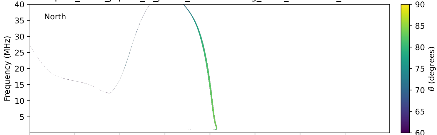
expres_earth_jupiter_io_jrm09_lossc-wid1deg_3kev_19900620_v11.cdf
