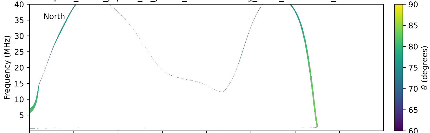
expres_earth_jupiter_io_jrm09_lossc-wid1deg_3kev_19900611_v11.cdf
