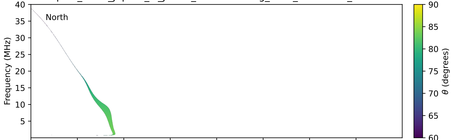
expres_earth_jupiter_io_jrm09_lossc-wid1deg_3kev_19900608_v11.cdf
